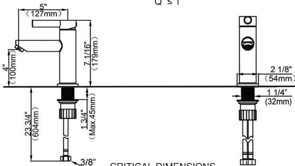
CRITICAL DIMENSIONS
